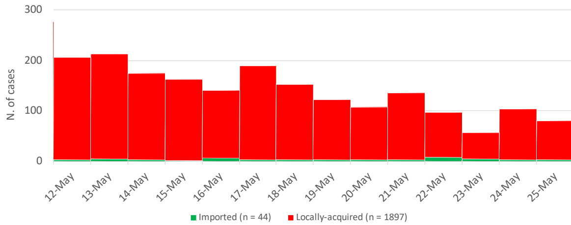
Figure A3A: Number of cases by origin of infection and by date of sample collection in the last 14 days (12 – 25 May, 2021).
