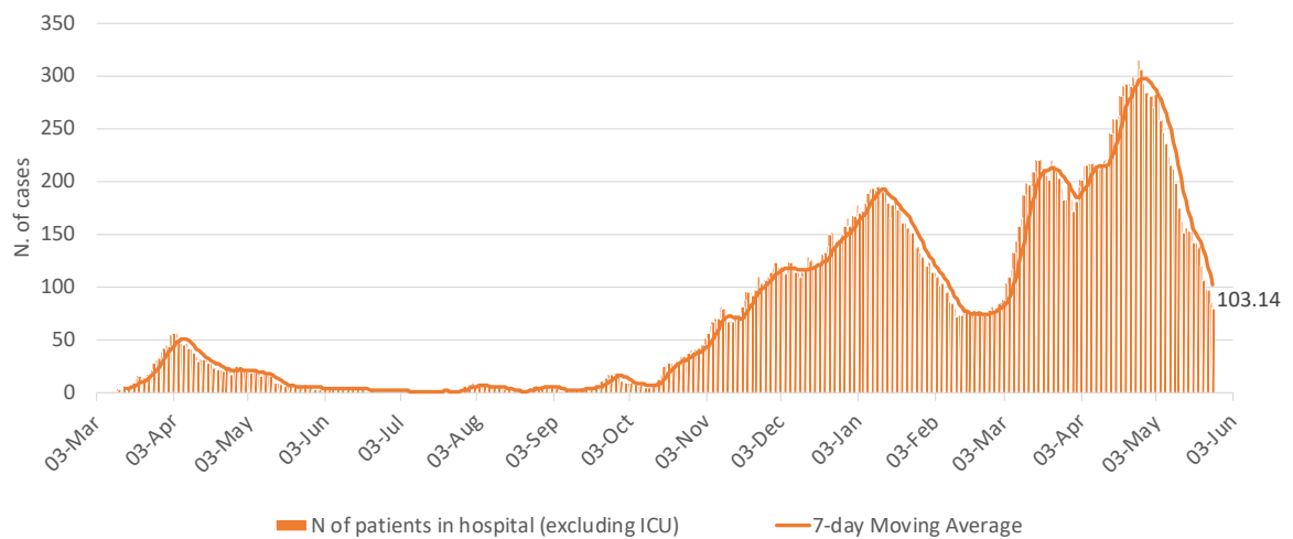
Figure 6b: Number and 7-day moving average (last moving average on May 26 th , 2021 is shown on the graph) of laboratory-confirmed COVID-19 cases in hospital every day (excluding those in ICU).
