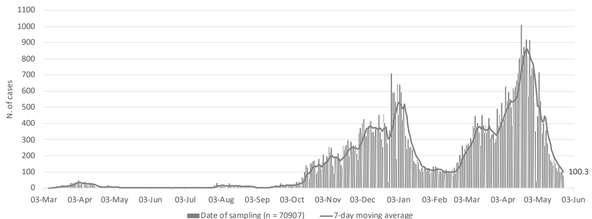
Figure 1: Number and 7-day moving average (last moving average on May 25 th , 2021, is shown on the graph) of laboratory-confirmed COVID-19 cases in the Republic of Cyprus since 03/03/2020 by date of sample collection*.
